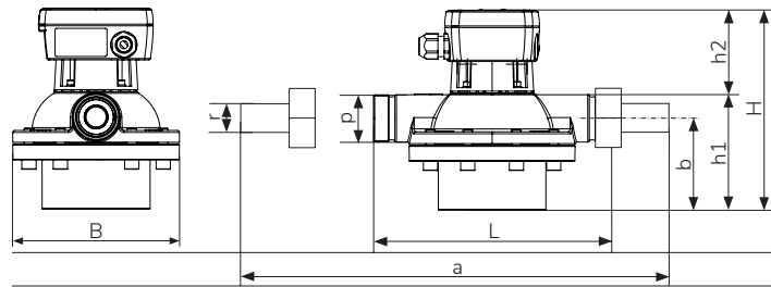
DN 40: with threaded ends
