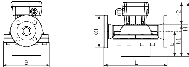
DN 40, 50: with flanges
