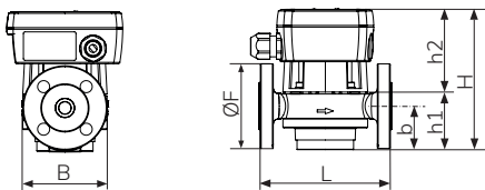
DN 15, 20, 25: with flanges
